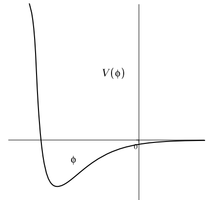
Figure 20: Effective potential for f(R) = R - R \ln R .
