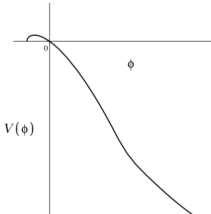
Figure 21: Effective potential for f(R) = R - 1/R , R > 0 .
