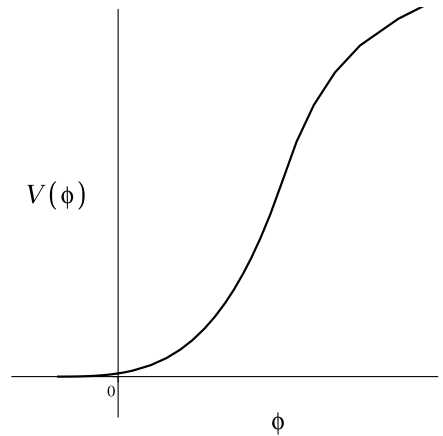
Figure 8: Effective potential for f(R) = R + R^{1.5} .
