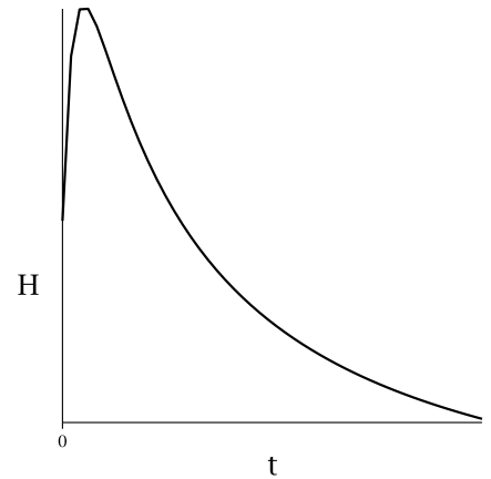
Figure 22: Stable numerical solution for f(R) = R - 1/R .
